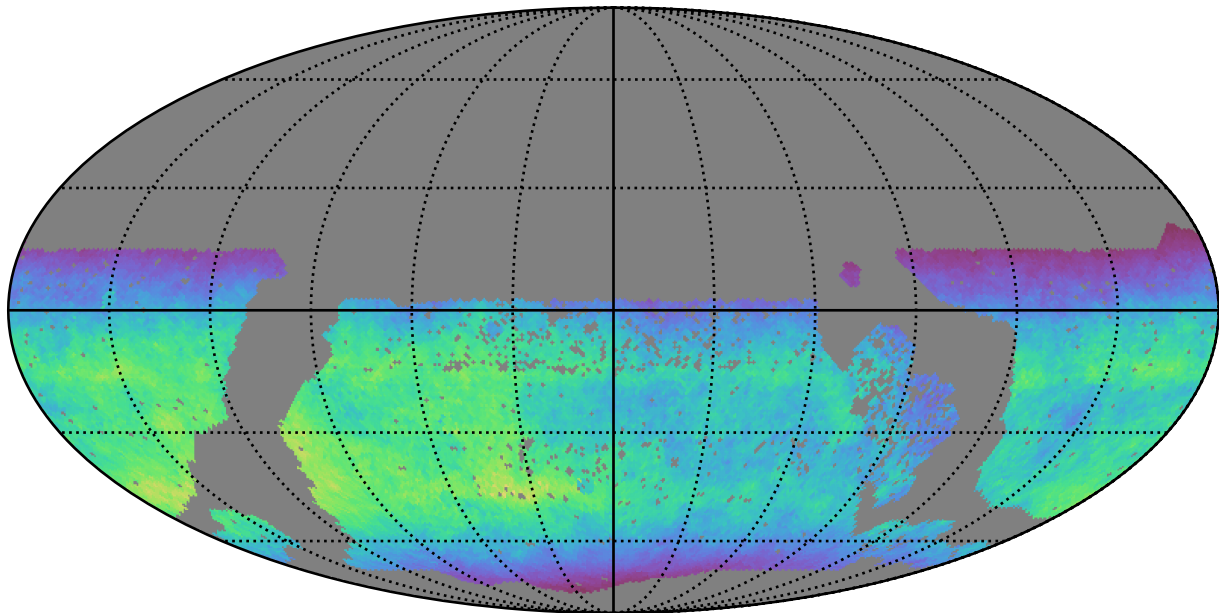
too_elab_r256_d3_griz_v3.4_10yrs WFD y band: Normalized Teff
