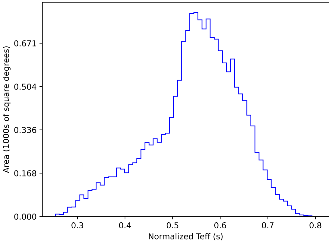
too_elab_r256_d3_griz_v3.4_10yrs WFD y band: Normalized Teff
