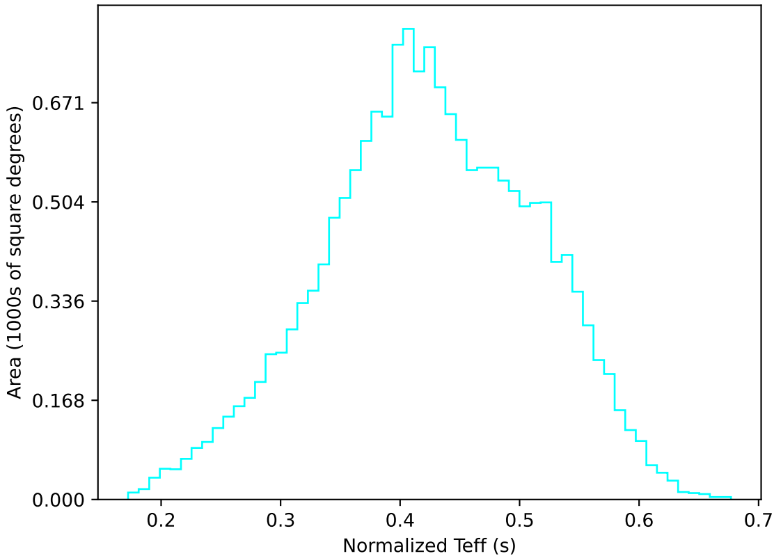
too_elab_r256_d3_griz_v3.4_10yrs WFD u band: Normalized Teff
