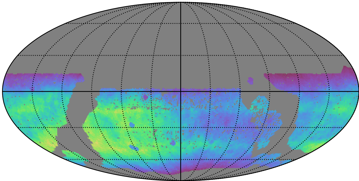
too_elab_r256_d3_griz_v3.4_10yrs WFD r band: Normalized Teff
