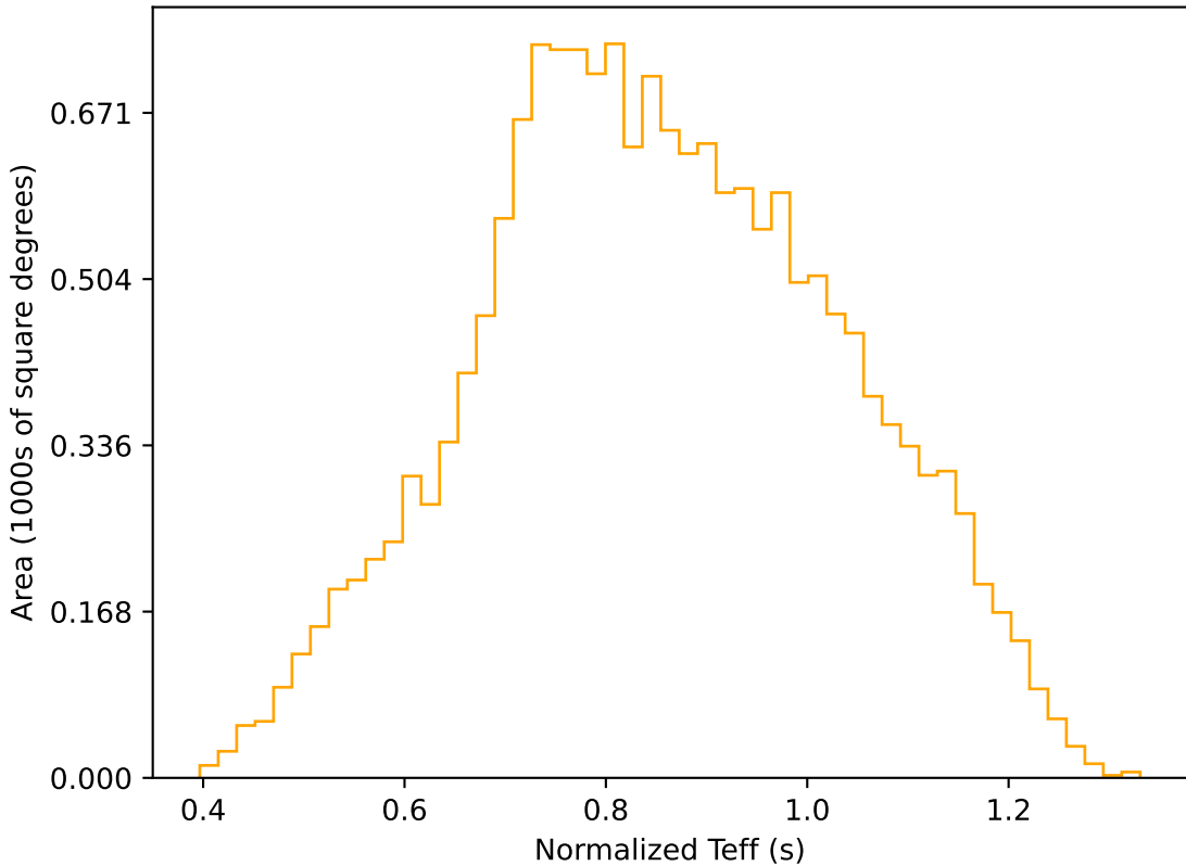
too_elab_r256_d3_griz_v3.4_10yrs WFD r band: Normalized Teff
