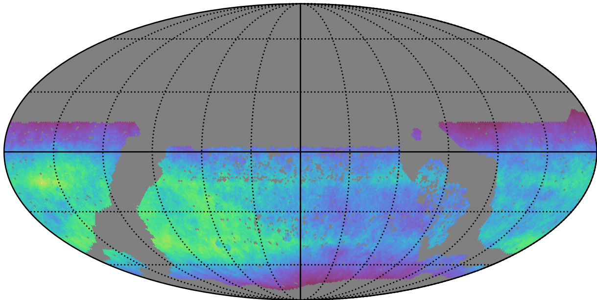
too_elab_r256_d3_griz_v3.4_10yrs WFD i band: Normalized Teff
