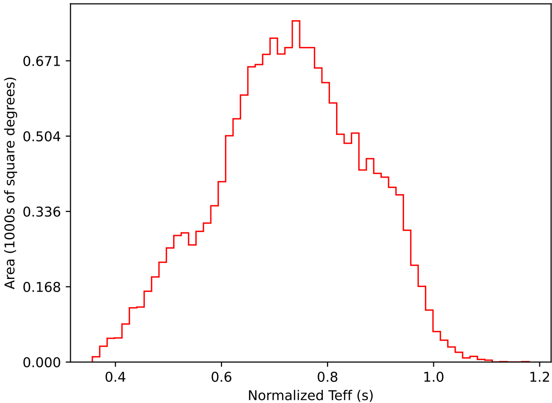
too_elab_r256_d3_griz_v3.4_10yrs WFD i band: Normalized Teff
