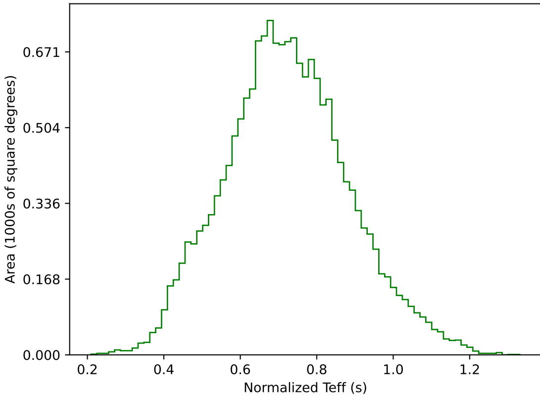
too_elab_r256_d3_griz_v3.4_10yrs WFD g band: Normalized Teff
