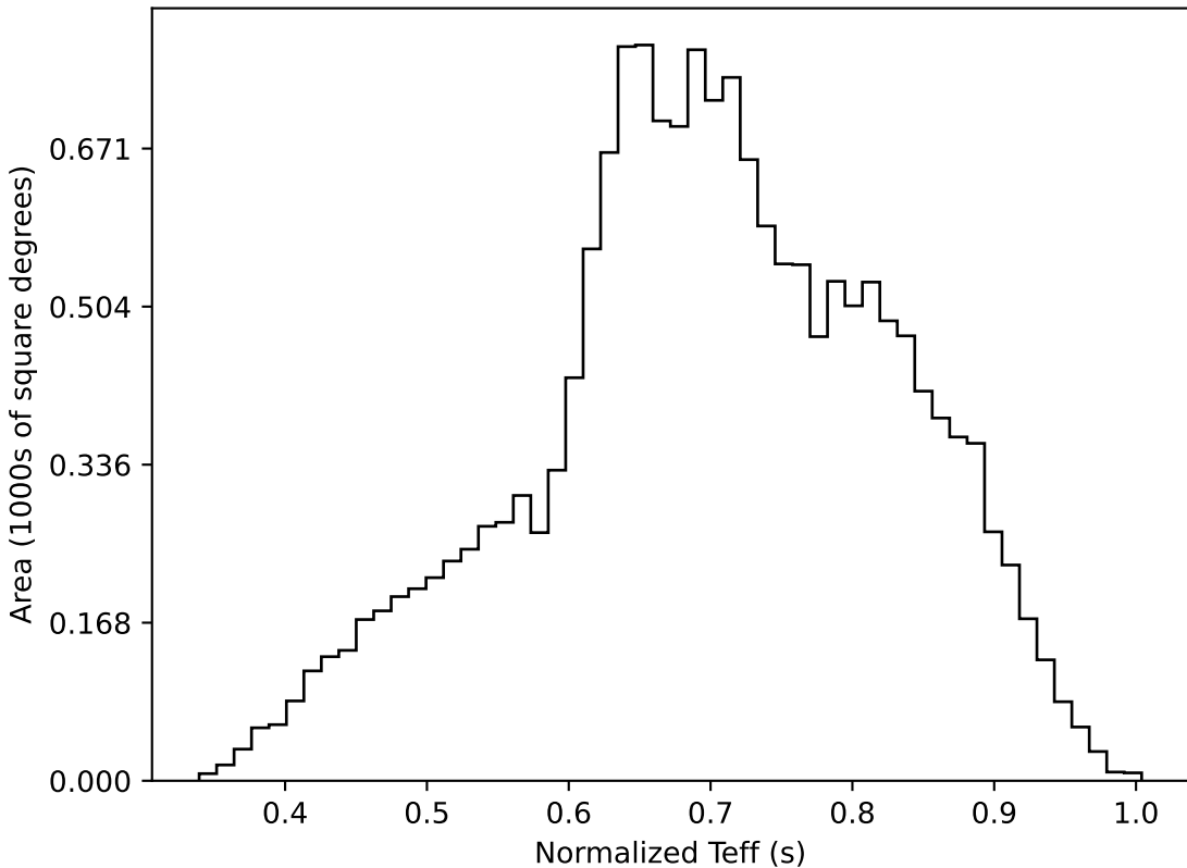
too_elab_r256_d3_griz_v3.4_10yrs WFD all bands: Normalized Teff
