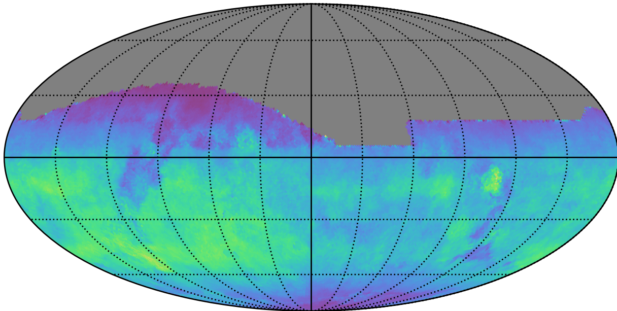
too_elab_r256_d3_griz_v3.4_10yrs All sky z band: Normalized Teff
