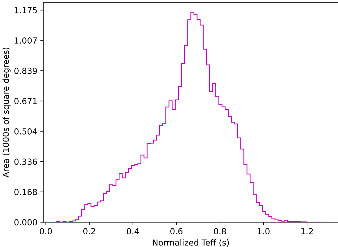
too_elab_r256_d3_griz_v3.4_10yrs All sky z band: Normalized Teff
