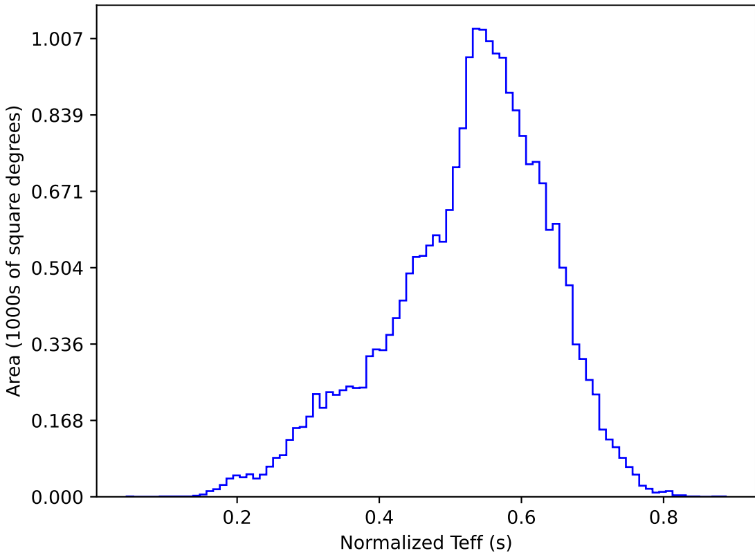
too_elab_r256_d3_griz_v3.4_10yrs All sky y band: Normalized Teff
