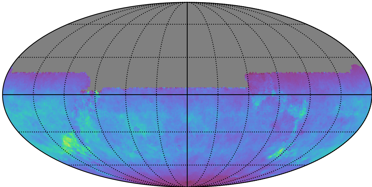
too_elab_r256_d3_griz_v3.4_10yrs All sky u band: Normalized Teff
