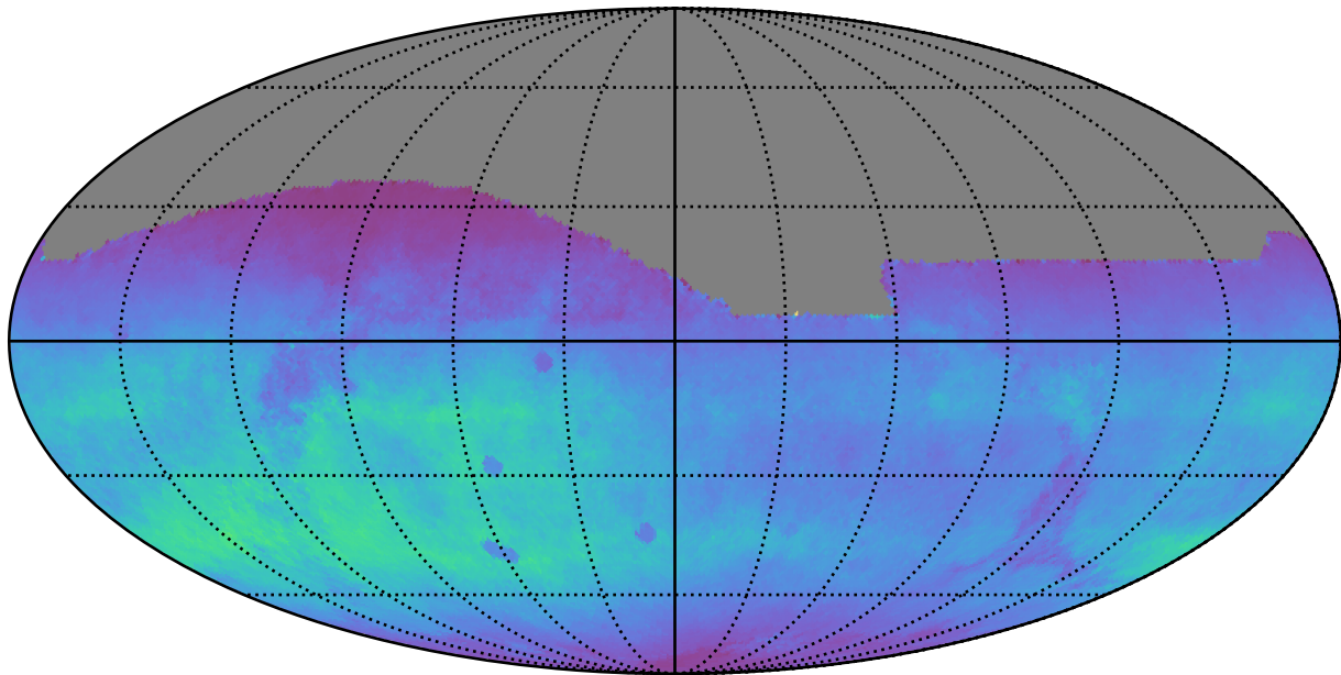
too_elab_r256_d3_griz_v3.4_10yrs All sky r band: Normalized Teff
