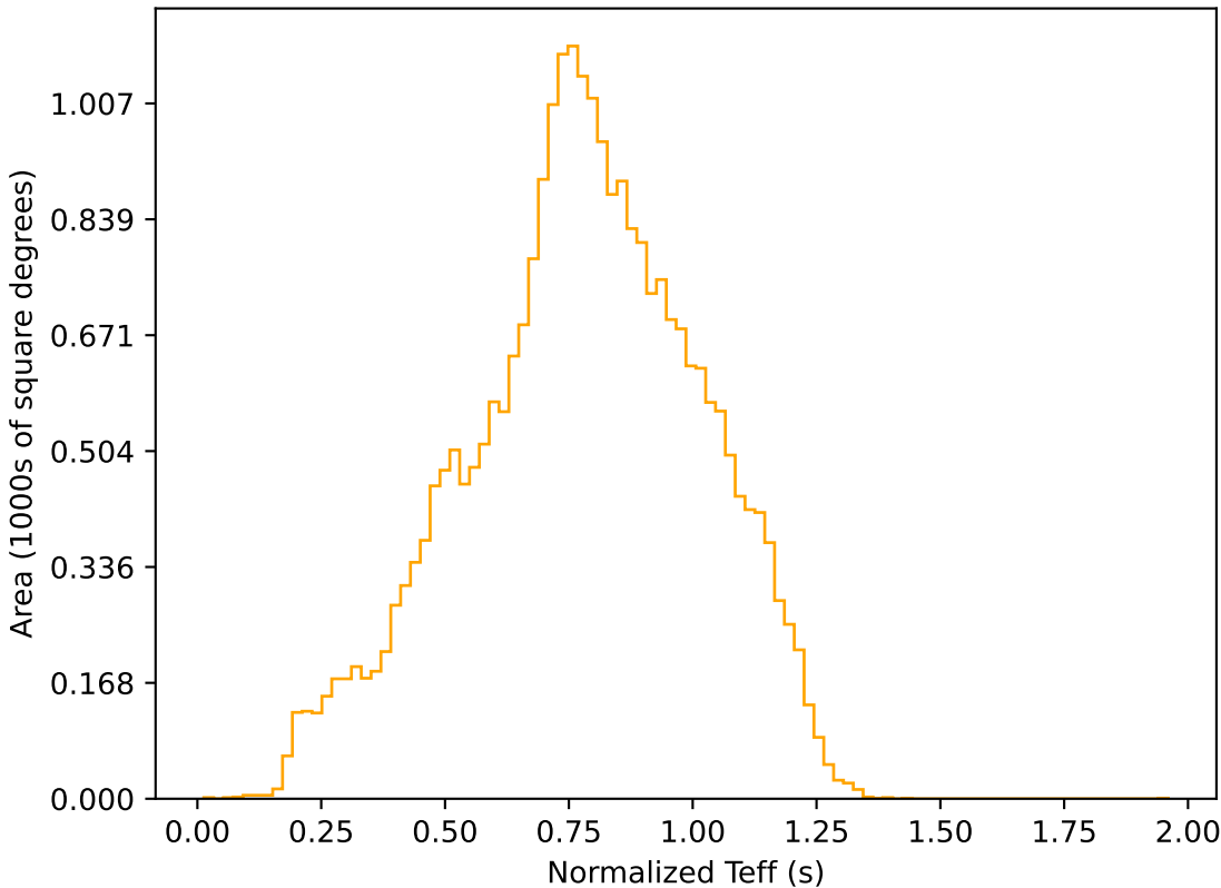
too_elab_r256_d3_griz_v3.4_10yrs All sky r band: Normalized Teff
