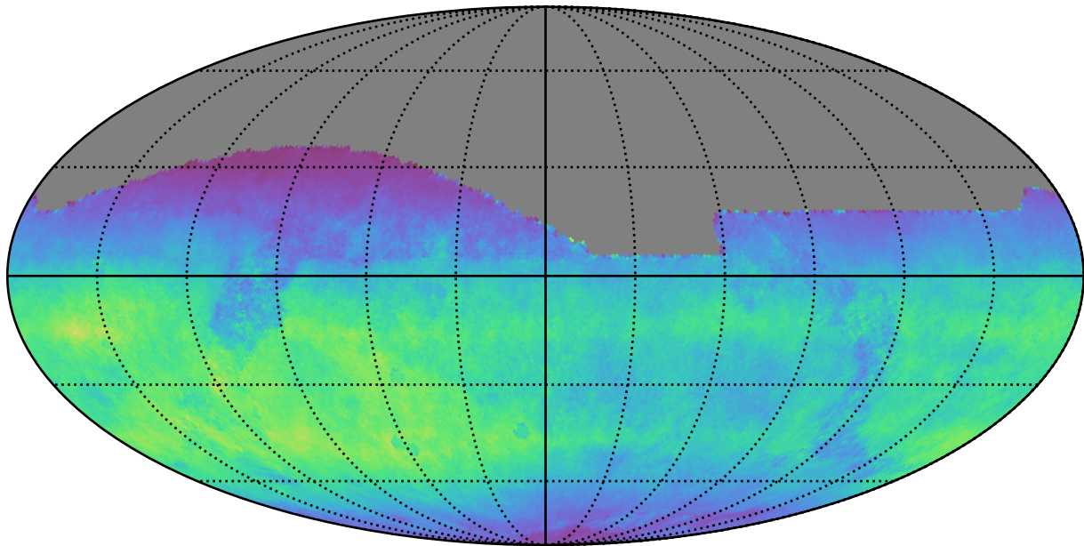
too_elab_r256_d3_griz_v3.4_10yrs All sky i band: Normalized Teff
