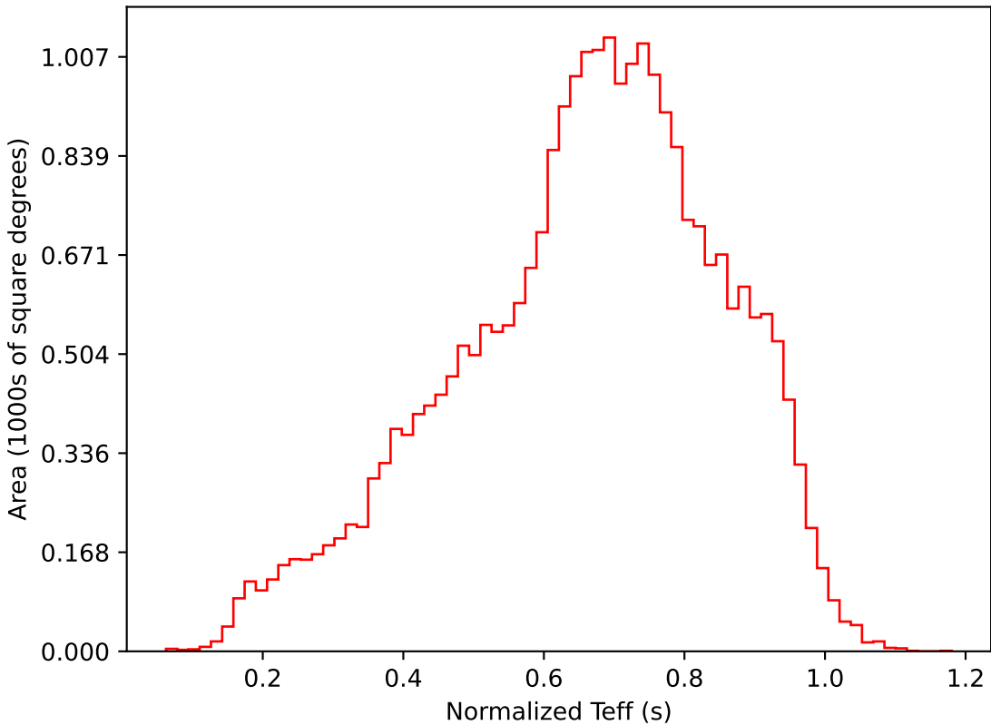
too_elab_r256_d3_griz_v3.4_10yrs All sky i band: Normalized Teff
