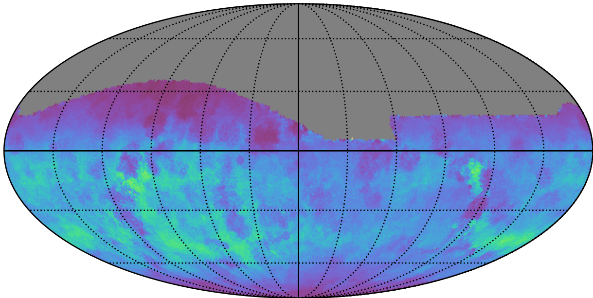
too_elab_r256_d3_griz_v3.4_10yrs All sky g band: Normalized Teff
