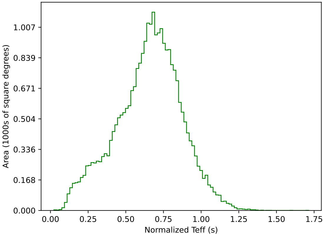
too_elab_r256_d3_griz_v3.4_10yrs All sky g band: Normalized Teff
