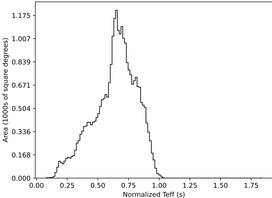
too_elab_r256_d3_griz_v3.4_10yrs All sky all bands: Normalized Teff
