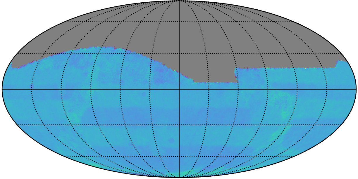
too_elab_r256_d3_griz_v3.4_10yrs All sky: Normalized Proper Motion Uncert @ 20.5
