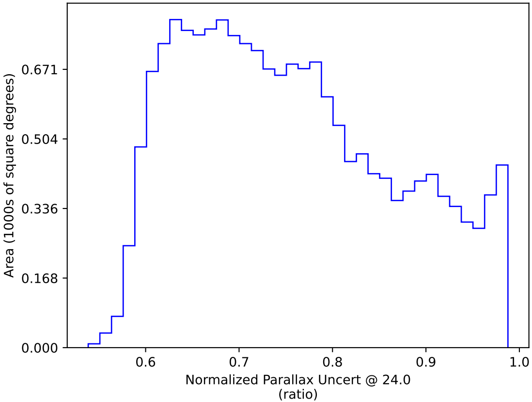
too_elab_r256_d3_griz_v3.4_10yrs WFD: Normalized Parallax Uncert @ 24.0
