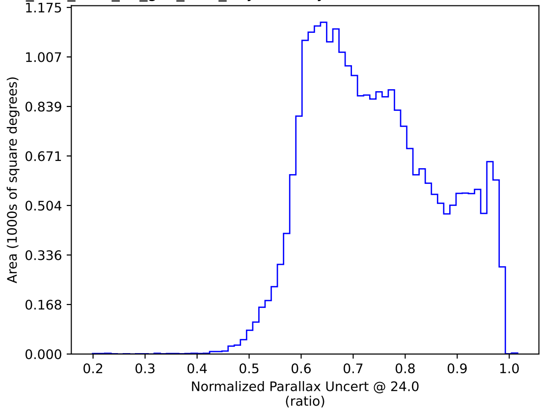
too_elab_r256_d3_griz_v3.4_10yrs All sky: Normalized Parallax Uncert @ 24.0
