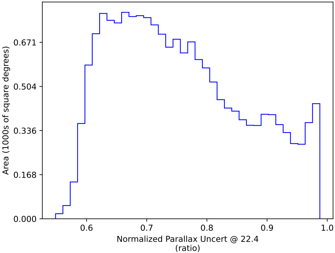
too_elab_r256_d3_griz_v3.4_10yrs WFD: Normalized Parallax Uncert @ 22.4
