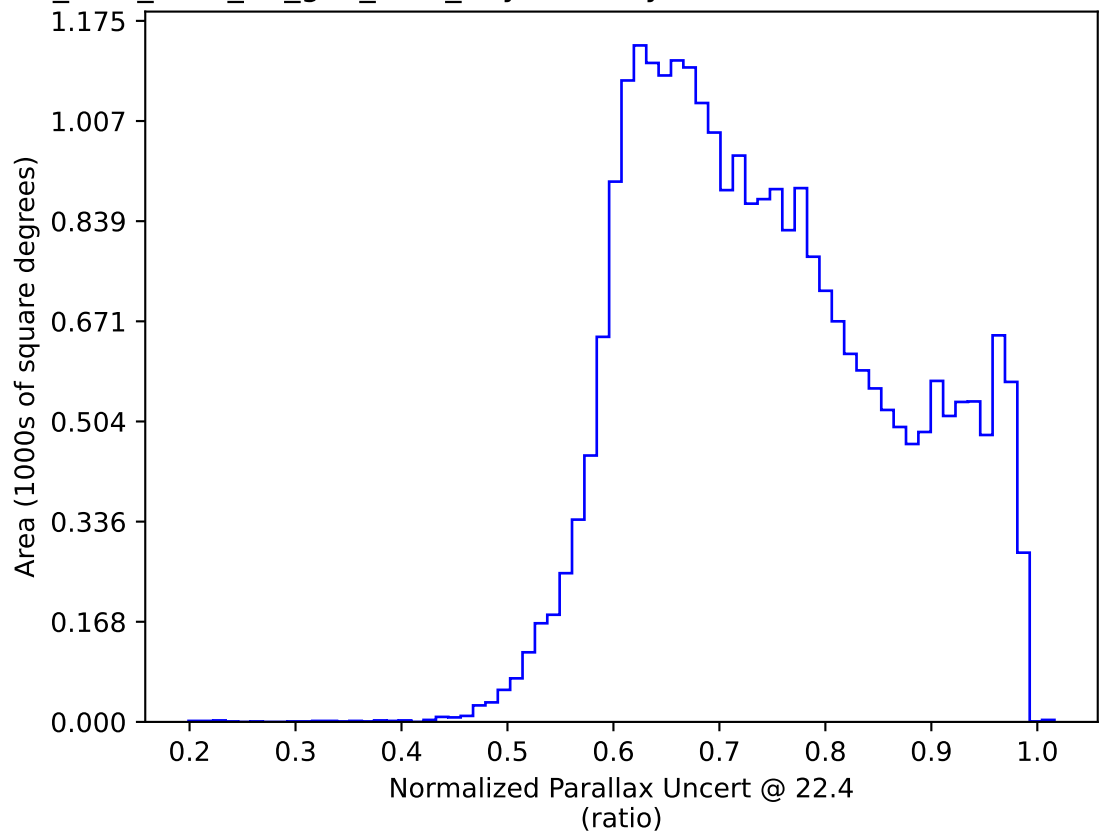
too_elab_r256_d3_griz_v3.4_10yrs All sky: Normalized Parallax Uncert @ 22.4
