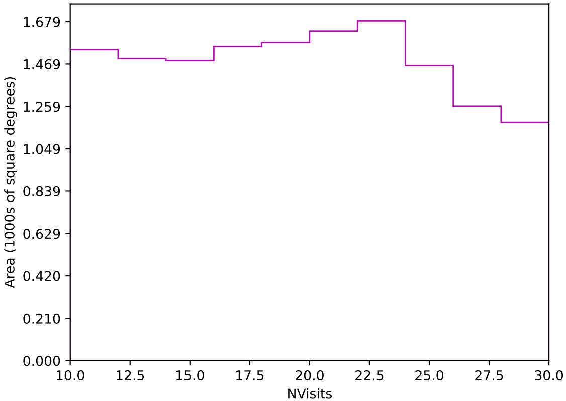
too_elab_r256_d3_griz_v3.4_10yrs Yr 3-4 z band: NVisits
