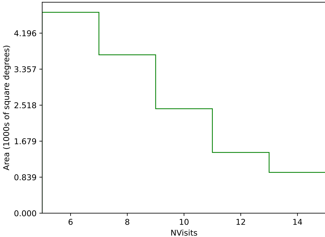
too_elab_r256_d3_griz_v3.4_10yrs Yr 3-4 g band: NVisits
