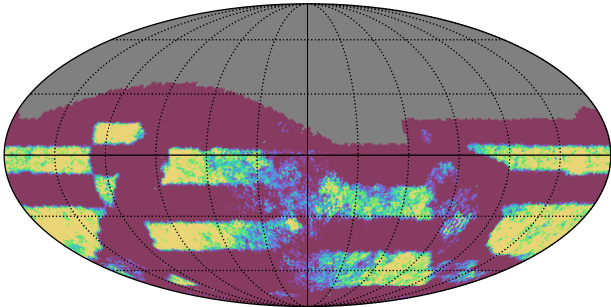
too_elab_r256_d3_griz_v3.4_10yrs Yr 3-4 all bands: NVisits
