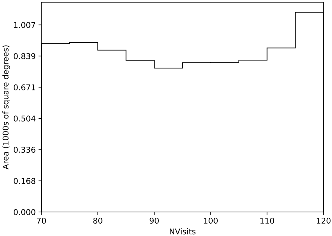
too_elab_r256_d3_griz_v3.4_10yrs Yr 3-4 all bands: NVisits
