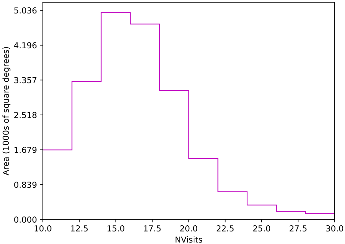
too_elab_r256_d3_griz_v3.4_10yrs Yr 1 z band: NVisits
