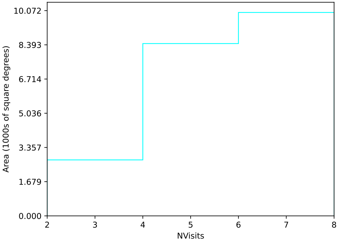
too_elab_r256_d3_griz_v3.4_10yrs Yr 1 u band: NVisits
