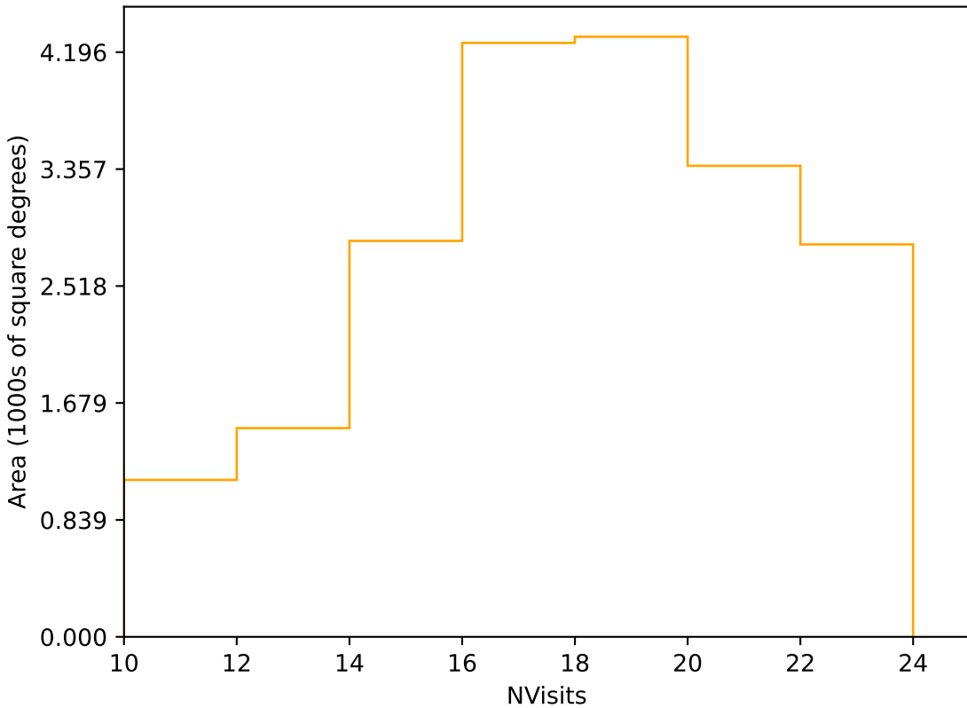
too_elab_r256_d3_griz_v3.4_10yrs Yr 1 r band: NVisits
