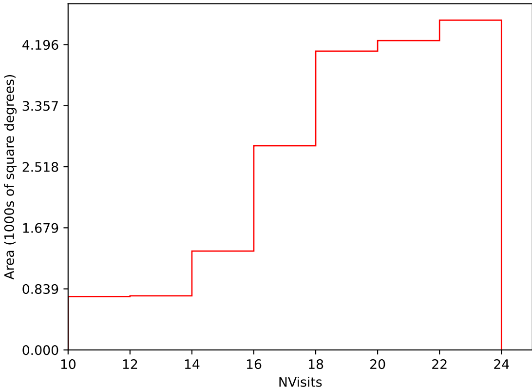
too_elab_r256_d3_griz_v3.4_10yrs Yr 1 i band: NVisits
