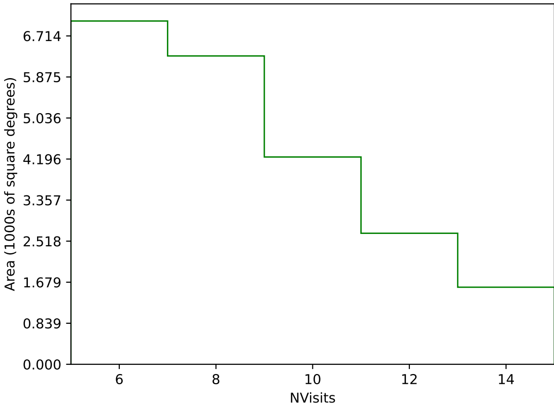
too_elab_r256_d3_griz_v3.4_10yrs Yr 1 g band: NVisits
