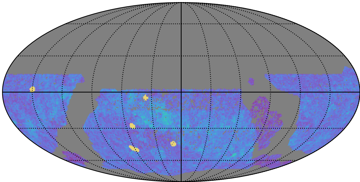
too_elab_r256_d3_griz_v3.4_10yrs WFD z band: NVisits
