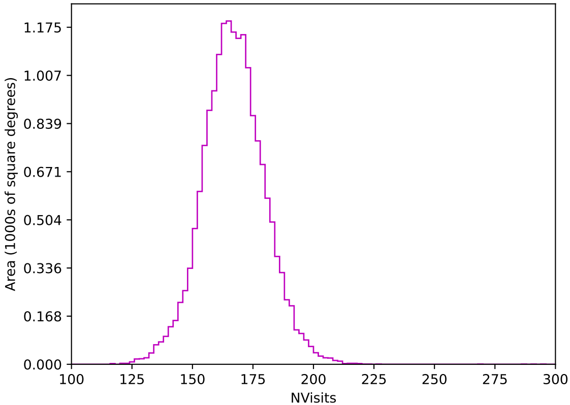
too_elab_r256_d3_griz_v3.4_10yrs WFD z band: NVisits
