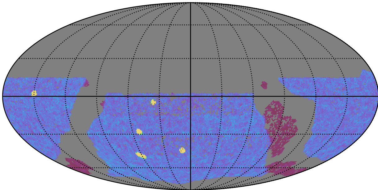
too_elab_r256_d3_griz_v3.4_10yrs WFD y band: NVisits
