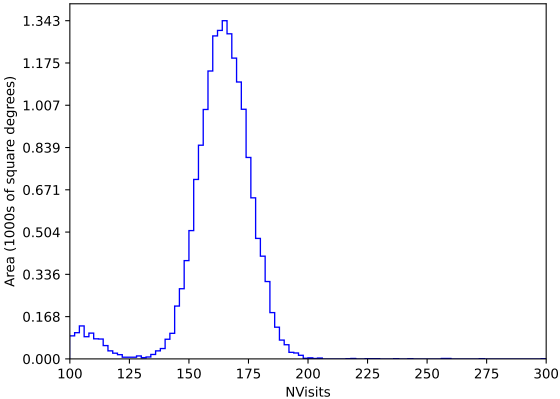
too_elab_r256_d3_griz_v3.4_10yrs WFD y band: NVisits
