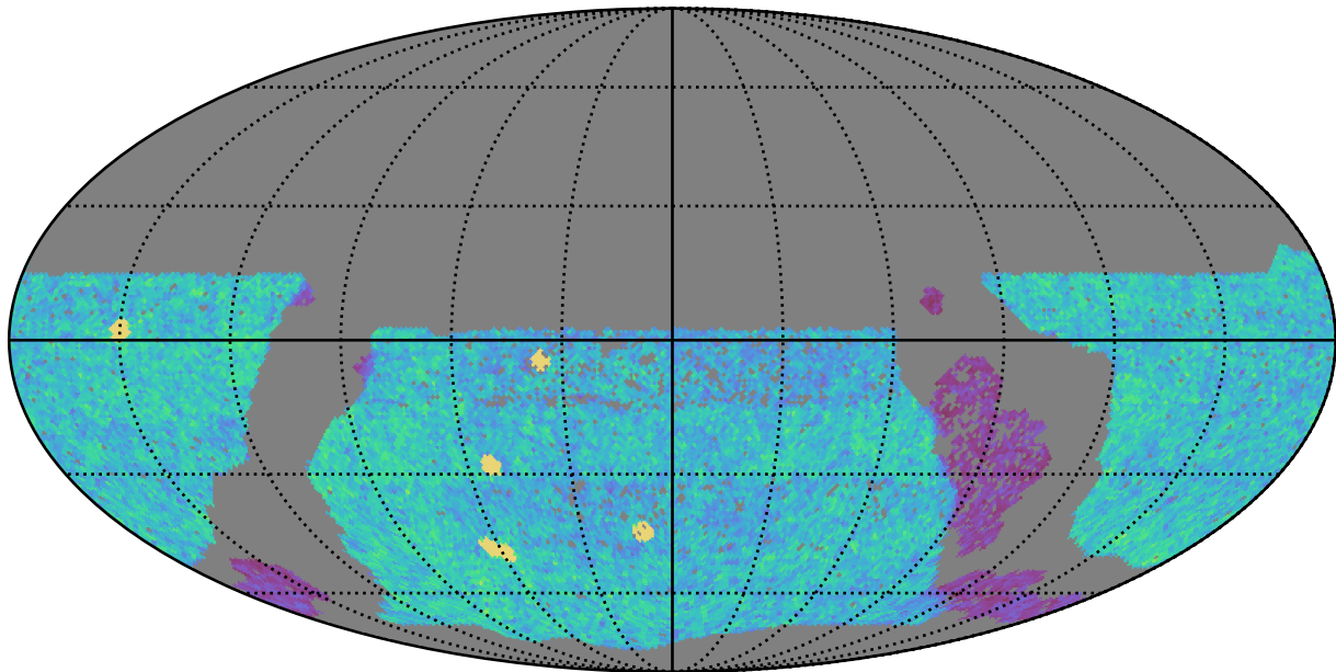
too_elab_r256_d3_griz_v3.4_10yrs WFD u band: NVisits
