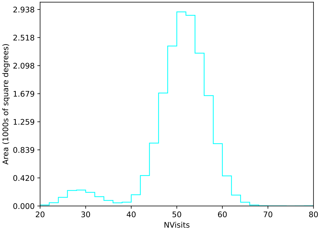
too_elab_r256_d3_griz_v3.4_10yrs WFD u band: NVisits
