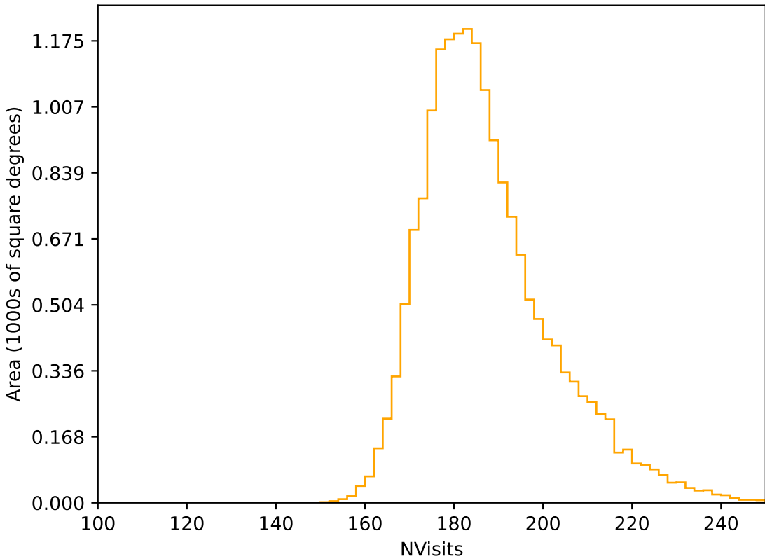
too_elab_r256_d3_griz_v3.4_10yrs WFD r band: NVisits
