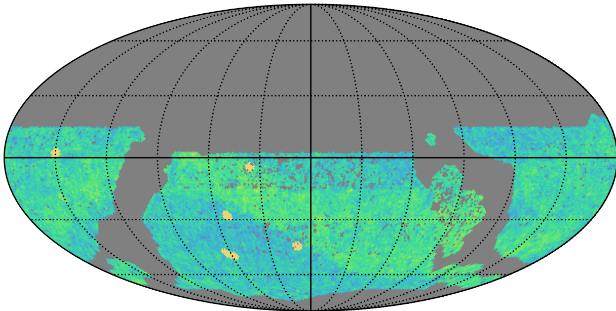
too_elab_r256_d3_griz_v3.4_10yrs WFD i band: NVisits
