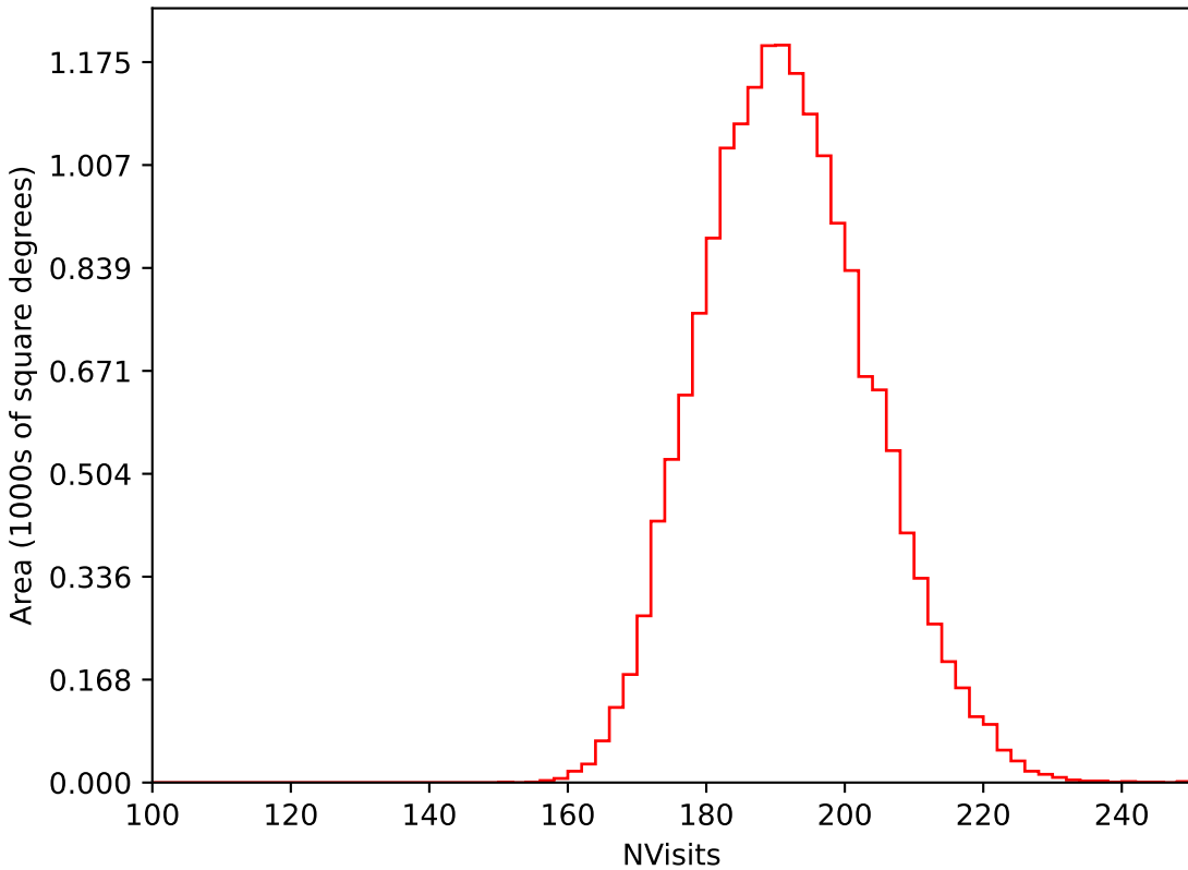
too_elab_r256_d3_griz_v3.4_10yrs WFD i band: NVisits
