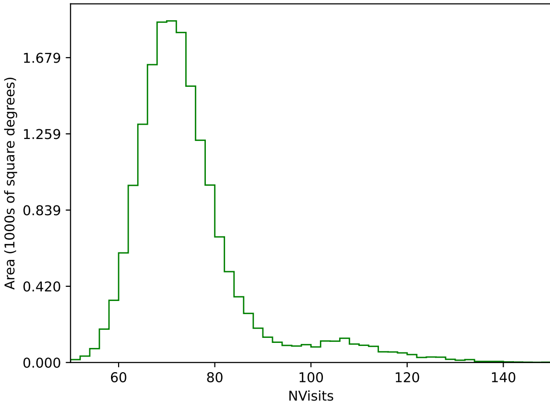
too_elab_r256_d3_griz_v3.4_10yrs WFD g band: NVisits
