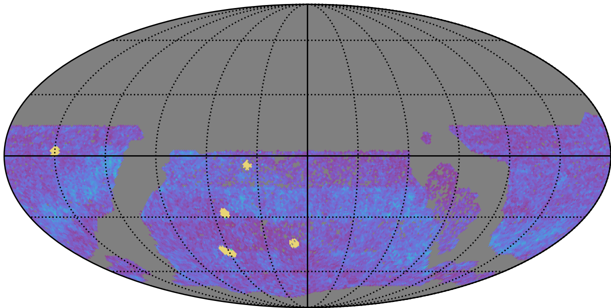
too_elab_r256_d3_griz_v3.4_10yrs WFD all bands: NVisits
