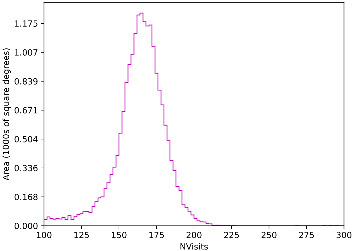
too_elab_r256_d3_griz_v3.4_10yrs All sky z band: NVisits
