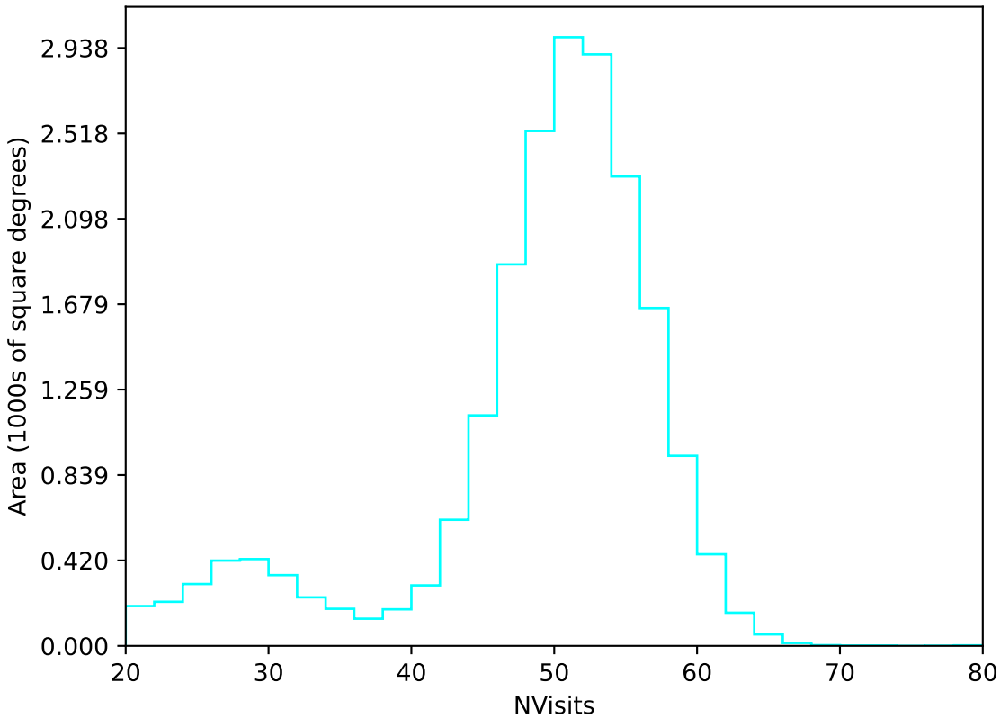
too_elab_r256_d3_griz_v3.4_10yrs All sky u band: NVisits
