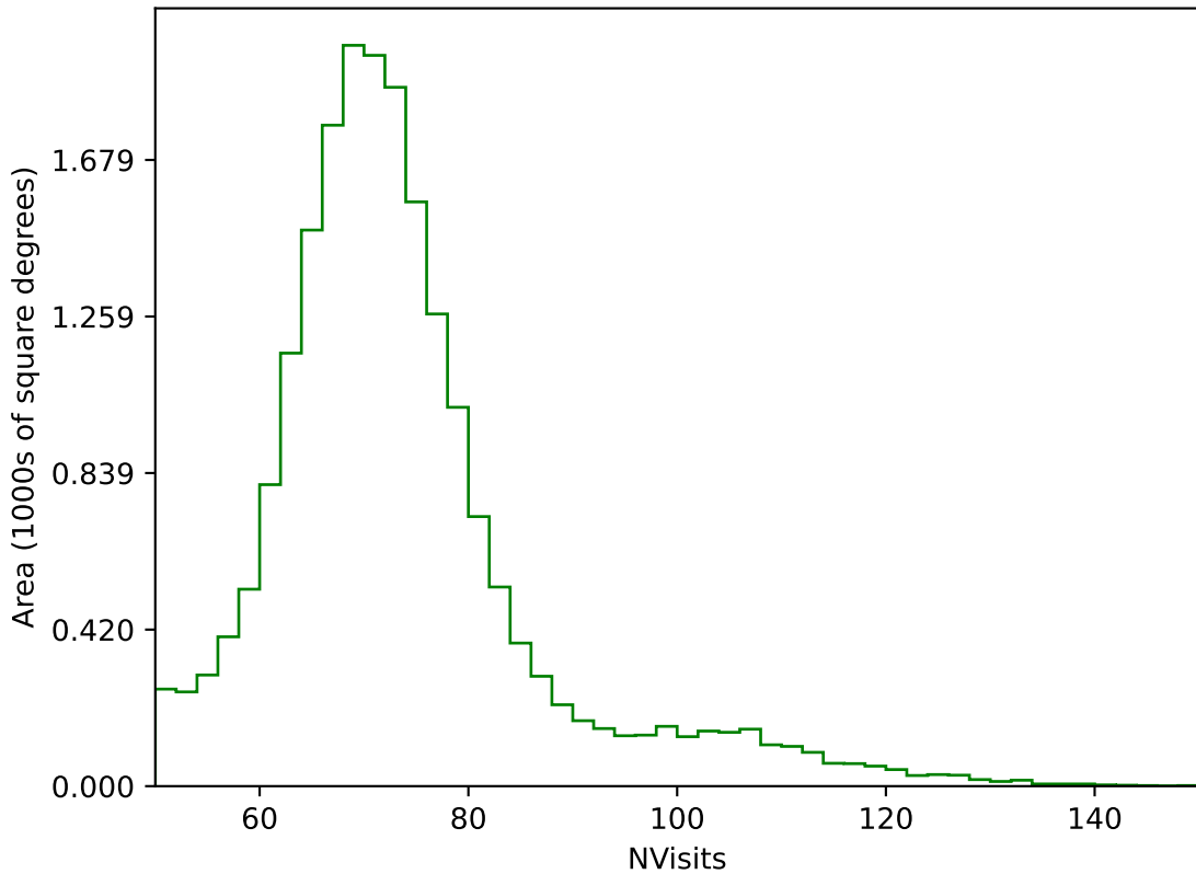
too_elab_r256_d3_griz_v3.4_10yrs All sky g band: NVisits
