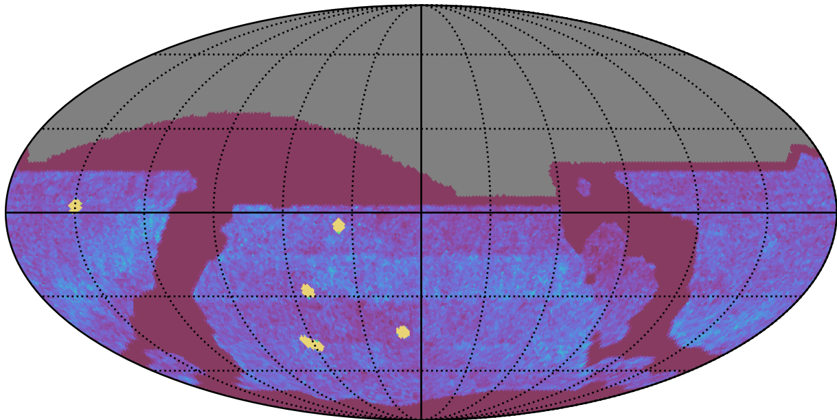
too_elab_r256_d3_griz_v3.4_10yrs All sky all bands: NVisits
