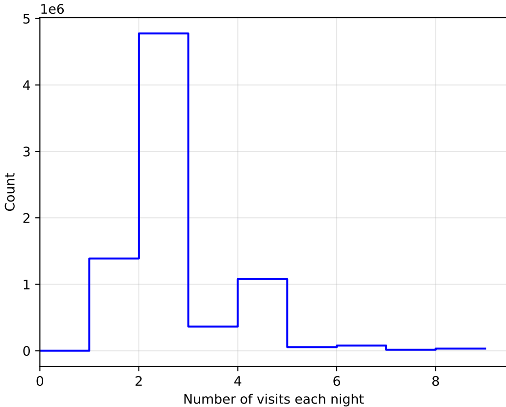
too_elab_r256_d3_griz_v3.4_10yrs WFD: NVisitsPerNight
